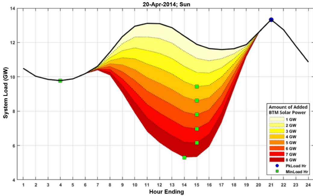
Figure 25: The “Duck Curve” in ISO New England [97]
