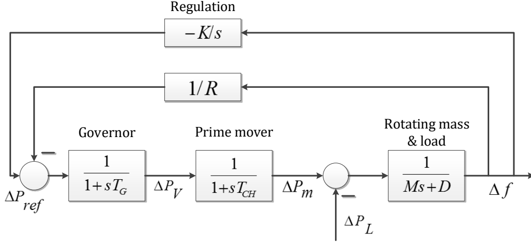
Figure 10: Power system automatic generation control [12]
