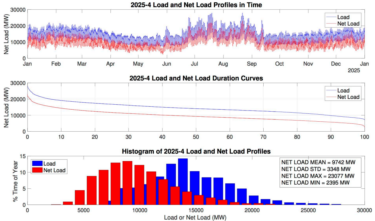
Figure 15: Comparison of load and net load for Scenario 2025-4
