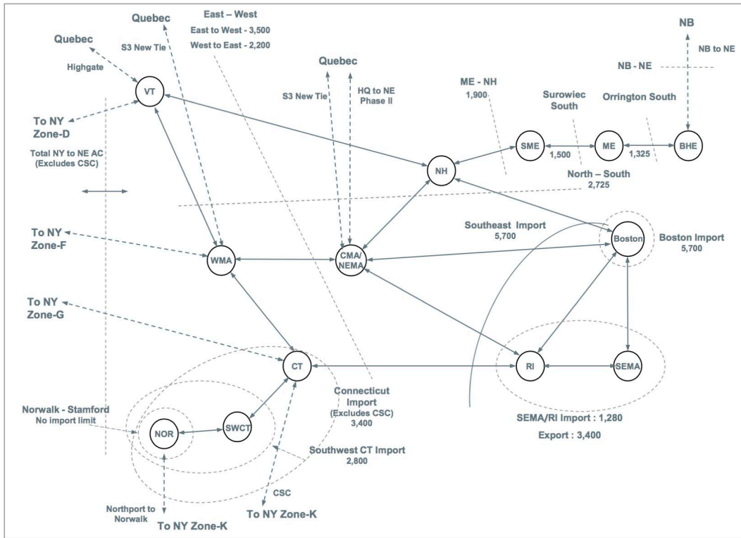
Figure 11: Topology of the ISO-NE zonal network model [42]
