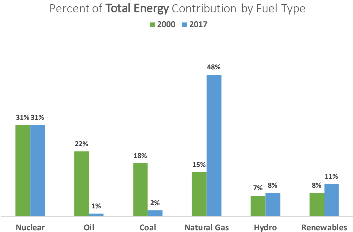
Figure 1: ISO New England generation mix in 2000 and 2017 [1].
