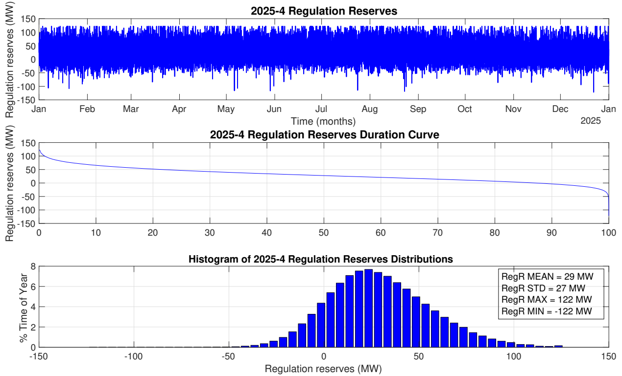
Figure 46: Regulation reserve performance for Scenario 2025-4
